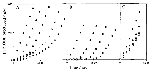
Figure 2. Inhibition of peroxidation of dilinoleoyl phosphatidylcholine by trolox, 4d, and 5i. Production of hydroperoxides from large multilamellar liposomes of dilinoleoyl phosphatidylcholine (20 mM) initiated by 2,2'-azobis-2,4-dimethylvaleronitrile (0.5 mM) at 48 °C. The conjugated diene formation was monitored at 234 nm. (A) (●) control experiment, ( \Delta ) trolox 2.5 \mu M, ( \square ) 5 \mu M, ( \circ ) 7.5 \mu M, ( \blacktriangle ) 10 \mu M; (B) (●) control experiment, ( \Delta ) 4d 16.6 \mu M, ( \square ) 33.3 \mu M, ( \circ ) 50 \mu M; (C) (●) control experiment, ( \Delta ) 5i 5 \mu M, ( \square ) 10 \mu M, ( \circ ) 15 \mu M. As on Figure 1, T_{inh} , R_{inh} , and R_p can be estimated.
